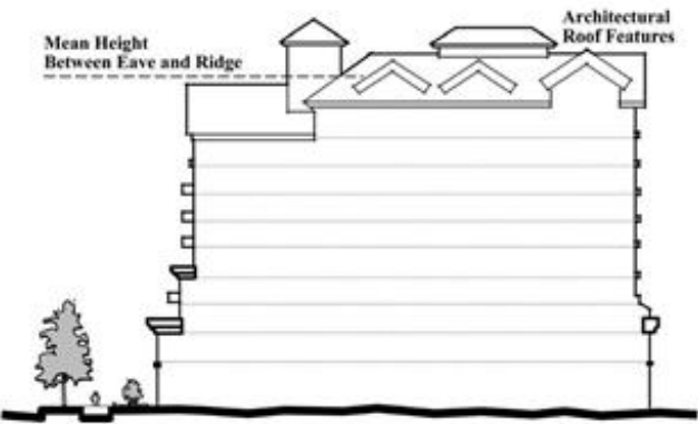
Figure 18.8 Measurement of Height Limits
