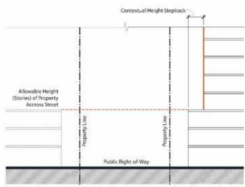
Figure 18.9 Contextual Height Stepbacks
